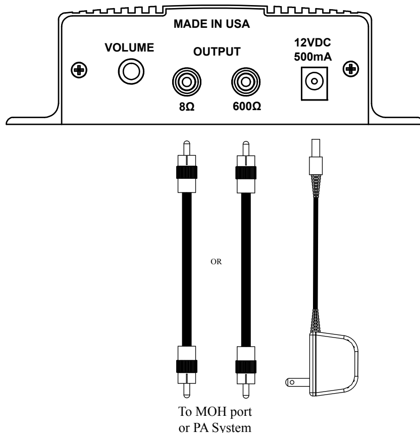
Wiring Diagram
